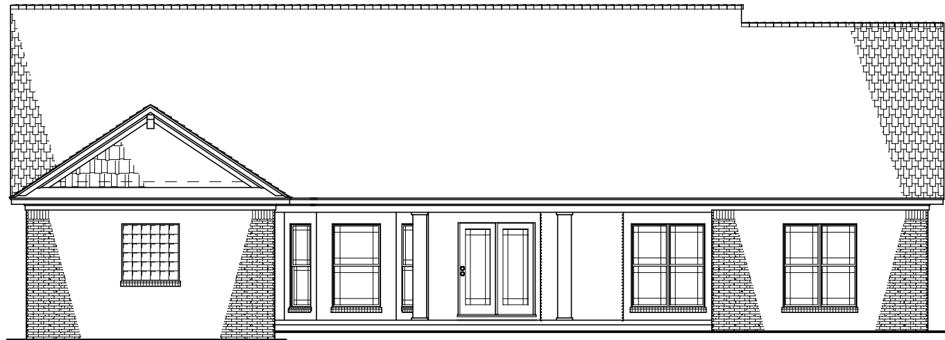
REAR ELEVATION
